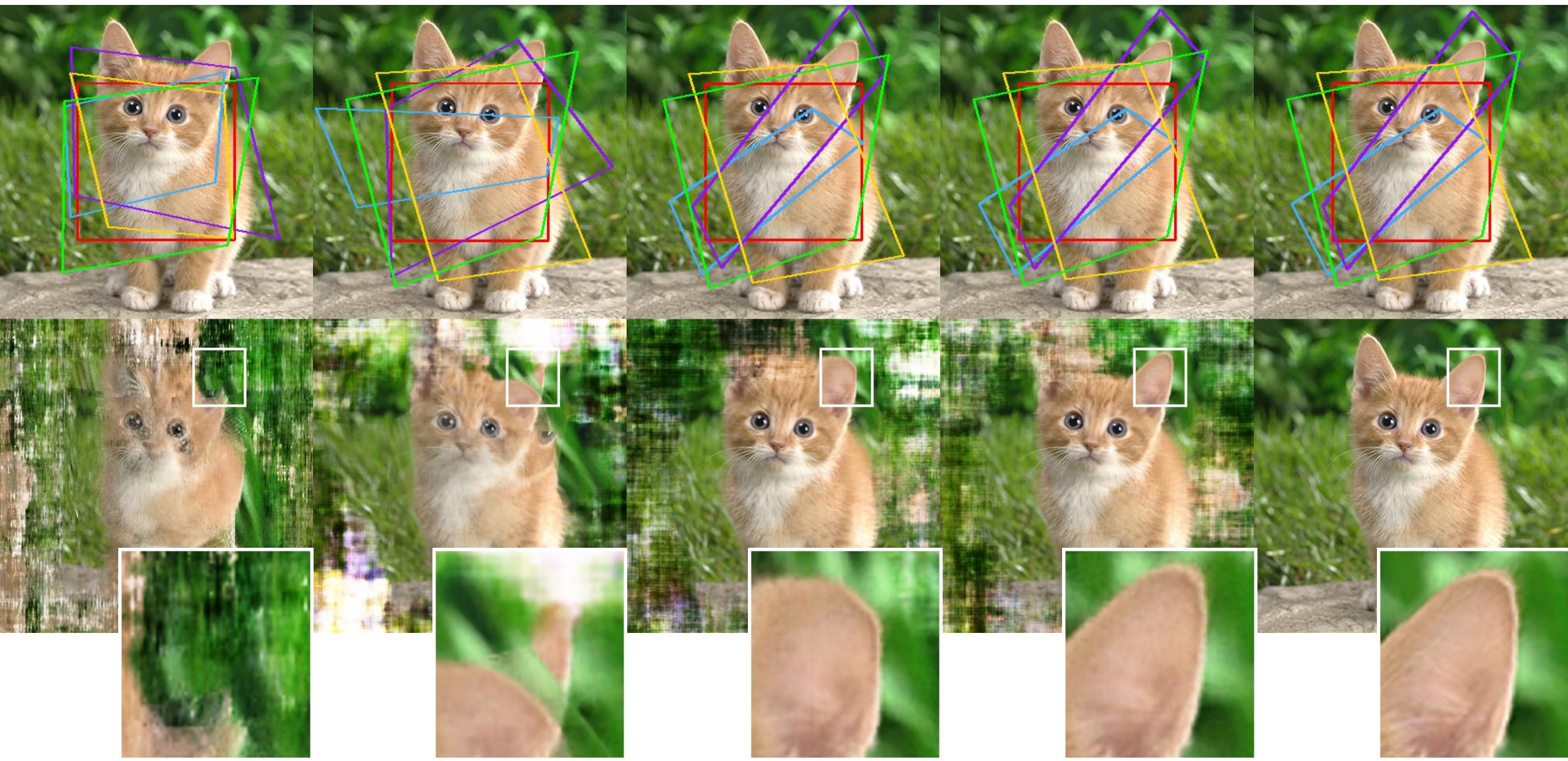
BARF (Global)
