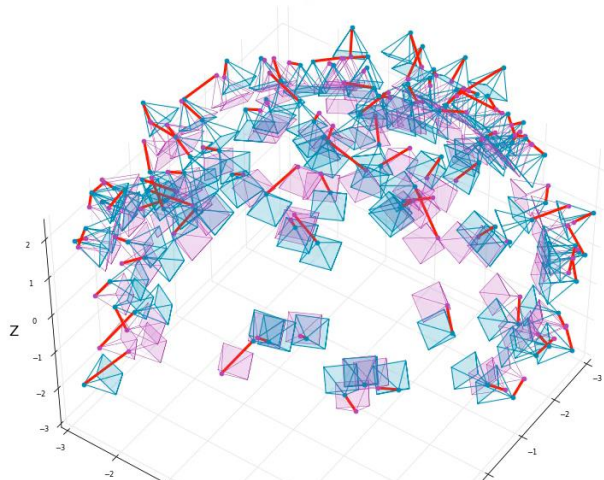
epoch 0
