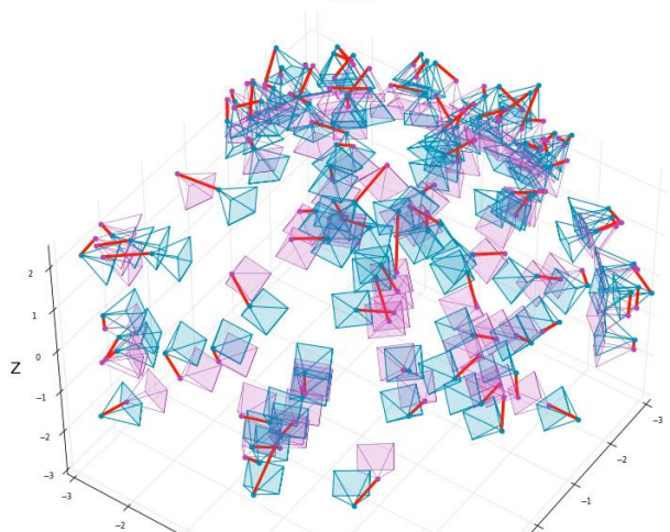
epoch 0
