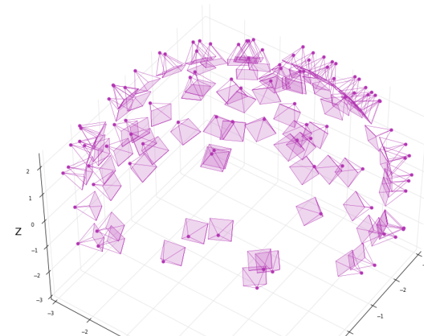
epoch 0
