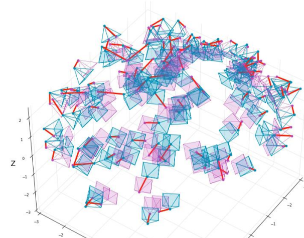
epoch 0
