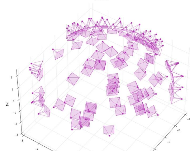
epoch 0
